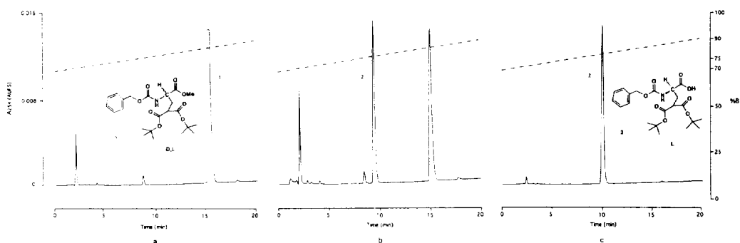
Fig. 1 HPLC profiles of the enzymatic saponification of L - \gamma -DL- tert -butyl-DL-Glu-OMe. Reaction progress: (a) initial, (b) after 20 h. Separation: (c) aqueous Na 2 CO 3 /NaHCO 3 layer. Reaction and extraction conditions in the main text. Chromatographic conditions: Column: Lichrosphere RP-18, 5 \mu m, 0.46 x 25 cm; solvent A: aqueous 0.10% TFA; solvent B: H 2 O/CH 3 CN (1:4) 0.08% TFA. Gradient elution from 70 to 90% B in 20 min. Flow: 1 ml/min. Detection: 215 nm.
